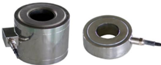
Compression : Model AR 500kg- 1, 3, 5, 10, 20,50, 100, 200, 300 ton
