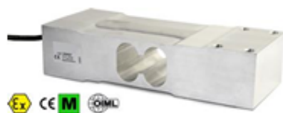
Single point : Model SPBC 100, 200, 300, 500, 630 kg
